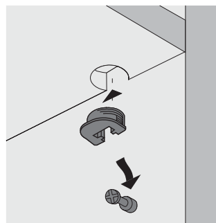
MDF 15mm
